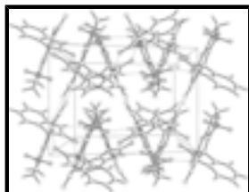
Fig. 2. A packing diagram of the title compound. Intermolecular hydrogen bonds are shown as dashed lines.
