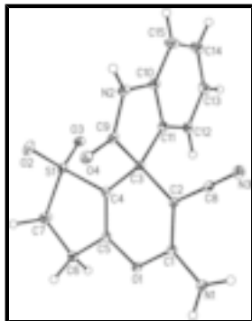
Fig. 1. The molecular structure of the title compound, showing 30% probability displacement ellipsoids and the atom-numbering scheme.
